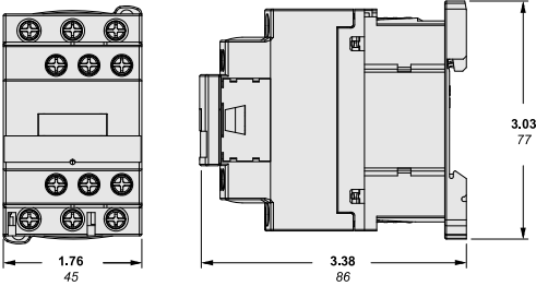
CONTACTOR WITH AC COIL
