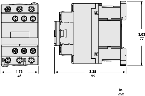
CONTACTOR WITH DC COIL
