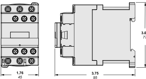
CONTACTOR WITH DC COIL
