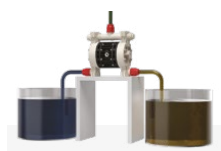
Split Suction
